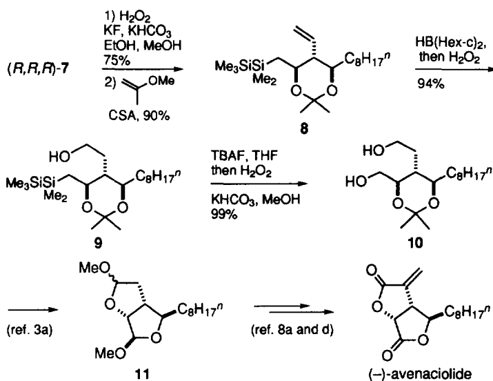
Scheme 1. Formal Total Synthesis of (–)-Avenaciolide.
